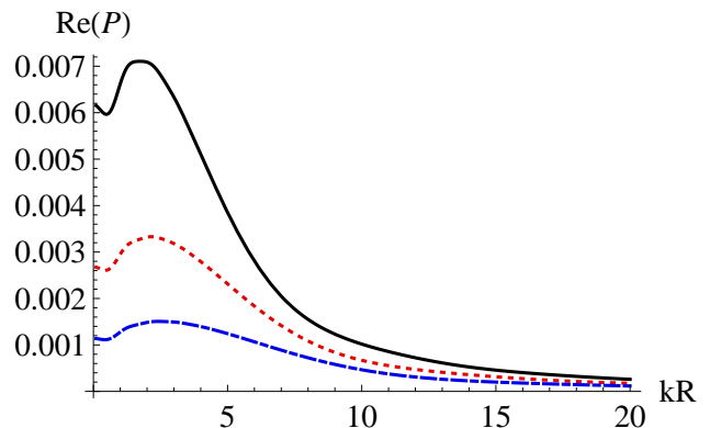
FIG. 9. (Color online) The power \frac{\Re[P]}{2\pi\rho_0 c v_0^2 R^2} of a rigid spherical cap moving with a constant velocity v_0 and various apertures, \theta_0 = 5\pi/32 (solid curve), \theta_0 = \pi/8 (dotted curve), and \theta_0 = \pi/10 (dashed-dotted curve), sphere radius R = 8.2 cm using Eqs. (10) and (39).
