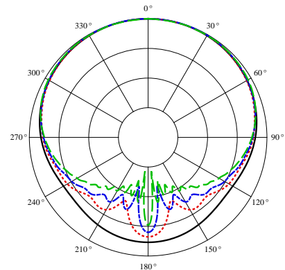
FIG. 6. (Color online) Polar plots of the SPL (10 dB/div.) of a simple source on a sphere of radius R=0.082 m. Frequency f = 1 kHz (solid curve), 4 kHz (dotted curve), 8 kHz (dashed-dotted curve), and 16 kHz (dashed curve), at distance r = 1 m, using Eqs. (25). All curves are normalized such that the SPL is 0 dB at \theta=0 .
