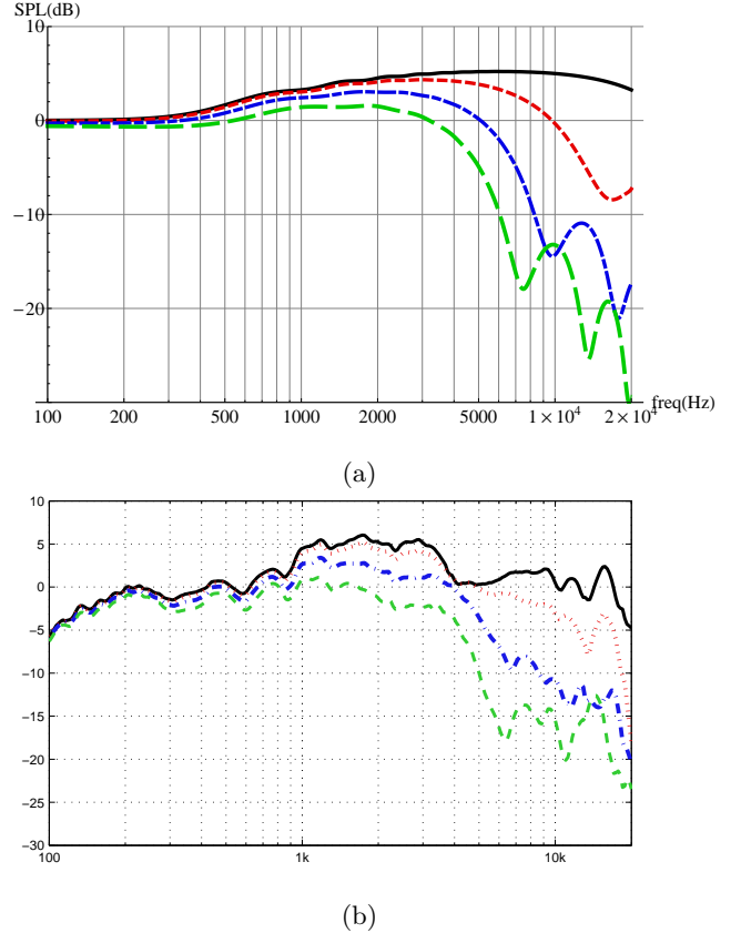
FIG. 5. (Color online) (a) Baffle step of a polar cap ( \theta_0 = \pi/8 ) on a sphere of radius R=0.082 m, \theta = 0 (solid curve), \theta = \pi/9 (dotted curve), \theta = 2\pi/9 (dashed-dotted curve), and \theta = 3\pi/9 (dashed curve), at distance r = 1 m, using Eqs. (21)–(23). All curves are normalized such that the SPL is 0 dB at 100 Hz. (b) Frequency response of a driver (same as Fig. 1-a, a = 3.2 cm) mounted in a square side of a rectangular cabinet with dimensions 13x13x18.6 cm, where the parameter is the observation angle \theta . The loudspeaker was measured in an anechoic room at 1 m distance. The on-axis response was normalized to 0 dB at 200 Hz, the other curves were normalized by the same amount.
