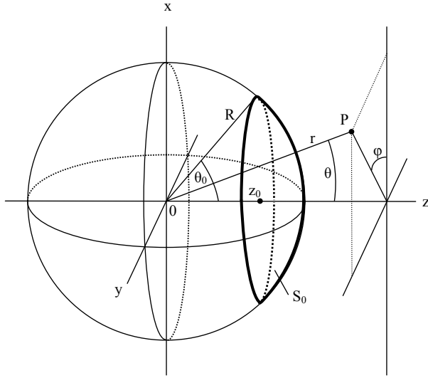
FIG. 2. Geometry and notations.
