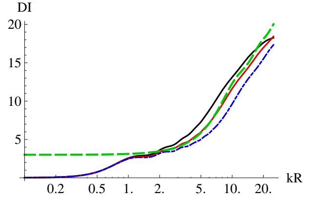
FIG. 11. (Color online) The directivity index DI = 10 \log_{10} D [dB] vs. kR (log. axis) of a rigid spherical cap with various apertures, \theta_0 = 5\pi/32 (solid curve), \theta_0 = \pi/8 (dotted curve), and \theta_0 = \pi/10 (dashed-dotted curve), and sphere radius R = 8.2 cm using Eqs. (10) and (49). The light-long-dashed curve starting at 3 dB is the directivity for a rigid piston in an infinite baffle, using Eq. (50). The logarithmic horizontal axis runs from kR=0.1 –25, corresponding to a frequency range from 66 Hz–16.5 kHz.
