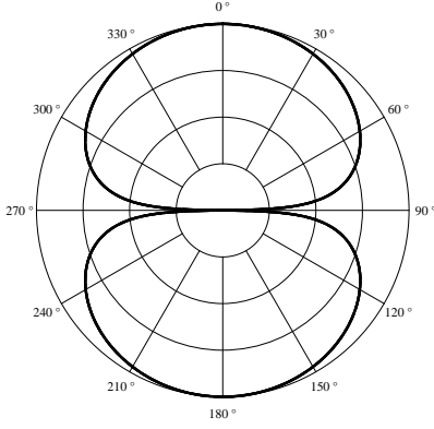
FIG. 4. Polar plot for a sphere ( \theta_0 = \pi ) moving with constant velocity V in the z -direction, using Eqs. (7) and (11). In this case W_1 = 1 , W_n is equal to zero for all values n \neq 1 .
