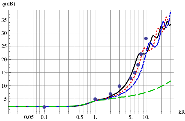
FIG. 12. (Color online) The function 20 \log_{10} |q| [dB] vs. kR (log. axis) given by Eq. (54) of a rigid spherical cap with various apertures, \theta_0 = 5\pi/32 (solid curve), \theta_0 = \pi/8 (dotted curve), and \theta_0 = \pi/10 (dashed-dotted curve), using Eqs. (7) and (11), and a simple source on a sphere using Eq. (25) (dashed curve), all at r = 1 m and sphere radius R = 8.2 cm. The solid circles are from a real driver (same as Fig. 1-a, a = 3.2 cm) mounted in a square side of a rectangular cabinet. The logarithmic horizontal axis runs from kR=0.02 –30, corresponding to a frequency range from 13 Hz–19.8 kHz.
