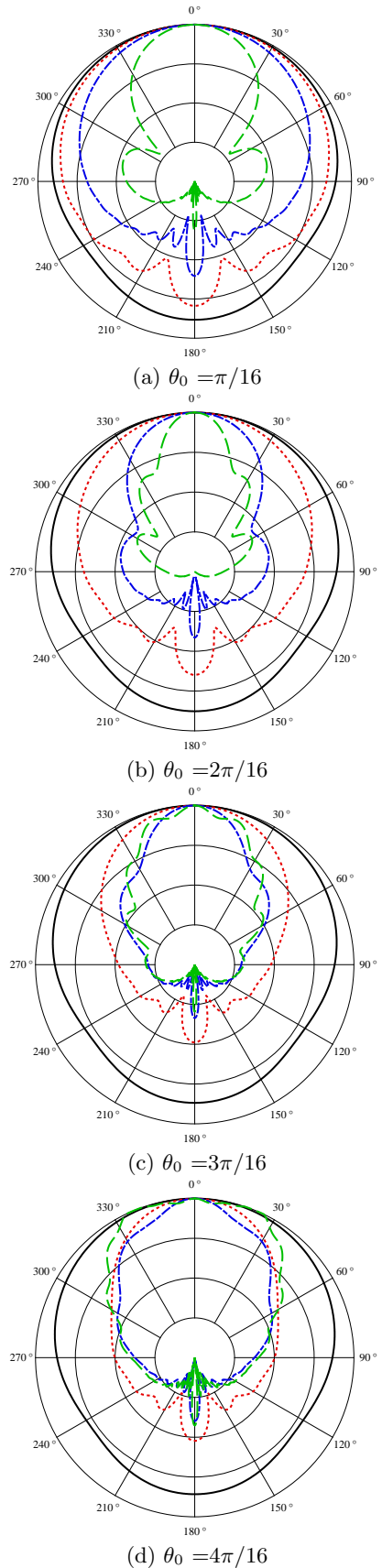
FIG. 3. (Color online) Polar plots of the SPL (10 dB/div.), f = 1 kHz (solid curve), 4 kHz (dotted curve), 8 kHz (dashed-dotted curve), and 16 kHz (dashed curve), Rigid spherical cap for various aperture \theta_0 , (sphere radius R = 8.2 cm, r = 1 m) using Eqs. (7) and (11). All curves are normalized such that the SPL is 0 dB at \theta = 0 .
