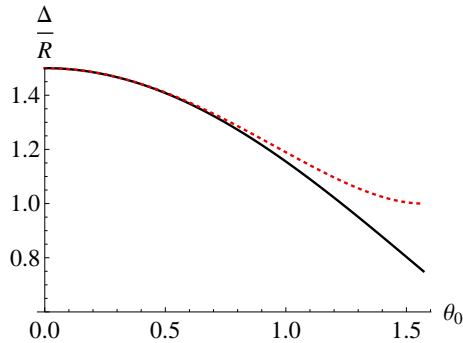
FIG. 13. (Color online) The relative acoustic center difference \Delta/R vs. \theta_0 using Eq. (64) for W is constant (solid curve) and using Eq. (65) for V is constant (dotted curve).
