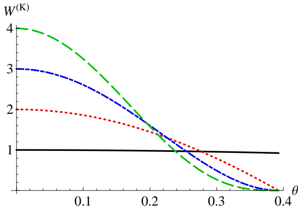
FIG. 7. (Color online) Stenzel profiles for K=0 (solid curve), K=1 (dotted curve), K=2 (dashed-dotted curve), and K=3 (dashed curve), using Eqs. (26) and (30) and \theta_0 = \pi/8 .
