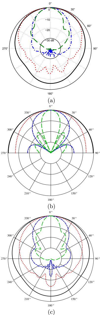
FIG. 1. (Color online) Polar plots of the SPL (10 dB/div.), f = 1 kHz (solid curve), 4 kHz (dotted curve), 8 kHz (dashed-dotted curve), and 16 kHz (dashed curve), corresponding for c = 340 m/s and a = 3.2 cm to ka values: 0.591, 2.365, 4.731, 9.462. All curves are normalized such that the SPL is 0 dB at \theta = 0 . (a) Loudspeaker radius a = 3.2 cm, measuring distance r = 1 m in rectangular cabinet, (b) Rigid piston ( a = 3.2 cm) in infinite baffle, (c) Rigid spherical cap (aperture \theta_0 = \pi/8 , sphere radius R = 8.2 cm, r = 1 m, corresponding to kR values: 1.5154, 6.0614, 12.1229, 24.2457) using Eqs. (7) and (11). The parameters a , R , and \theta_0 are such—using Eq. (13)—that the area of the piston and the cap are equal.
