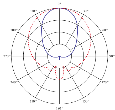
FIG. 15. (Color online) Polar plots (10 dB/div.) in the near field (solid curve, r = 0.0975 m) and in the far field (dotted curve, r = 1 m), corresponding to the parameters of the simulation example and the velocity profile of Fig. 14. All curves are normalized such that the SPL is 0 dB at \theta=0 .
