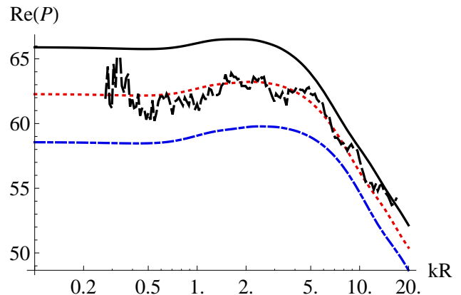
FIG. 10. (Color online) The power \frac{\Re[P]c}{2\pi\rho_0 a_0^2 R^4} [dB] vs. kR (log. axis) of a rigid spherical cap moving with a constant acceleration and various apertures, \theta_0 = 5\pi/32 (solid curve), \theta_0 = \pi/8 (dotted curve), and \theta_0 = \pi/10 (dashed-dotted curve), sphere radius R = 8.2 cm using Eqs. (10) and (39), together with power from the measured loudspeaker (dashed-irregular curve). The logarithmic horizontal axis runs from kR=0.1-20 , corresponding to a frequency range from 66 Hz–13.2 kHz.
