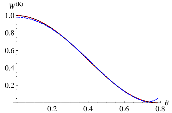
FIG. 14. (Color online) Stenzel profile W^{(K)}/(K+1) ( K = 2 and \theta_0 = \pi/4 ) of Eq. (72) using Eq. (20) directly (solid curve) together with the reconstructed profiles \hat{W}^{(K)} without noise (dotted curve) and with noise added to the pressure points \hat{p}_j (dashed-dotted curve). The (noiseless) reconstructed profile (dotted curve) coincides with the input profile (solid curve).
