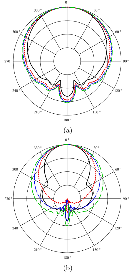
FIG. 8. (Color online) Polar plots of the SPL (10 dB/div.) of a spherical cap ( \theta_0 = \pi/8 , R = 8.2 cm, r = 1 m) with various Stenzel velocity profiles, K=0 (solid curve), K=1 (dotted curve), K=2 (dashed-dotted curve), and K=3 (dashed curve). (a) f = 4 kHz, (b) f = 8 kHz. All curves are normalized such that the SPL is 0 dB at \theta=0 .
